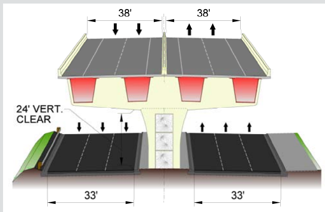
INTEGRAL SINGLE COLUMN PIER
