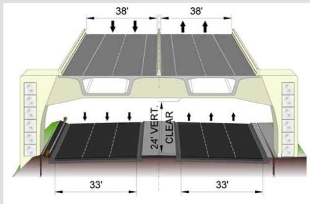
INTEGRAL STRADDLE PIER
